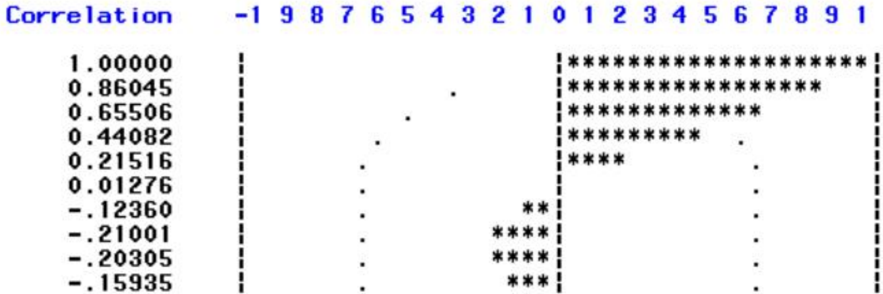
Autocorrelations
